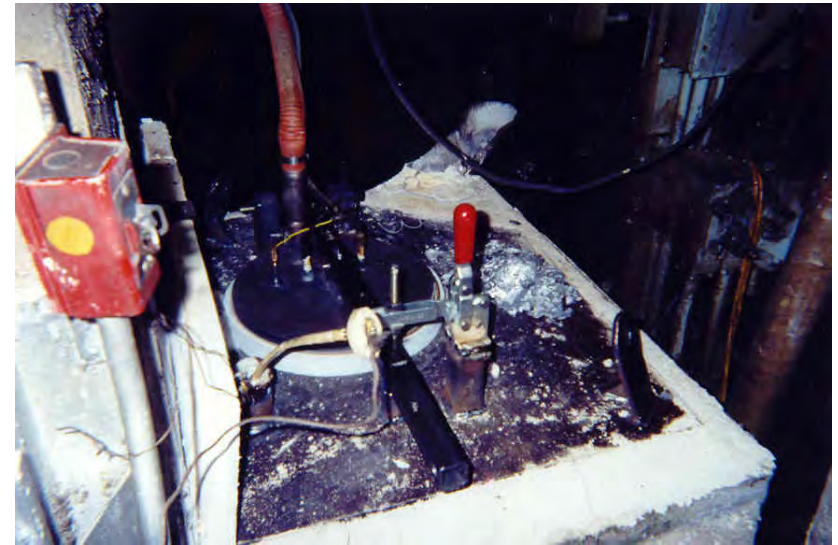
Ceramite® CSA Crucible in pump well position. Low pressure die cast operation.
